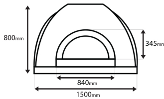
Oven Diagram (Front)
